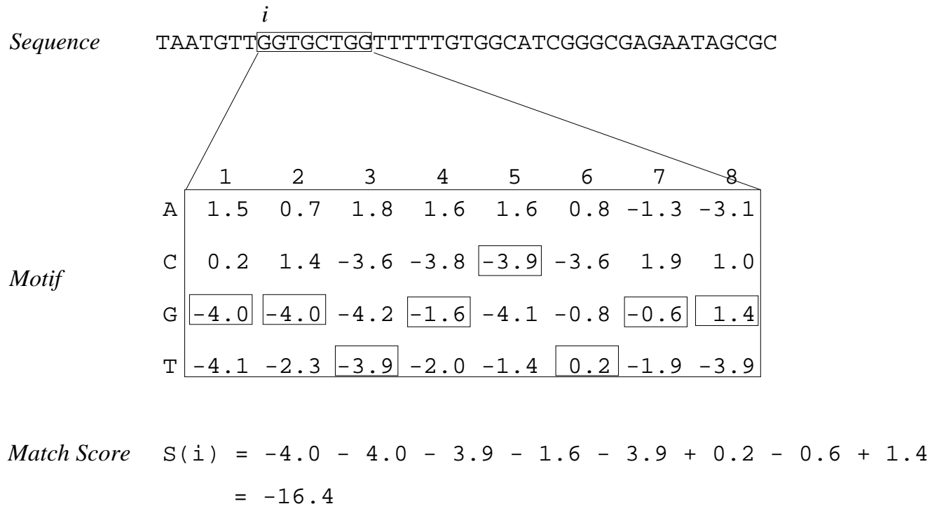
Figure 1: Computing motif match scores. The motif in this example represents a sequence pattern eight positions wide and hence contains eight columns of scores. Each column contains scores for matching each of the four letters in the DNA alphabet (ACGT) to that position in the motif. The subsequence starting at position i is GGTGCTGG, so the match score for position i in the sequence is determined by summing the score for G in position 1, G in position 2, T in position 3, etc., as shown in the illustration. The procedure for protein motifs is identical except that the protein alphabet contains twenty letters, and protein motifs consequently contain twenty rows.
