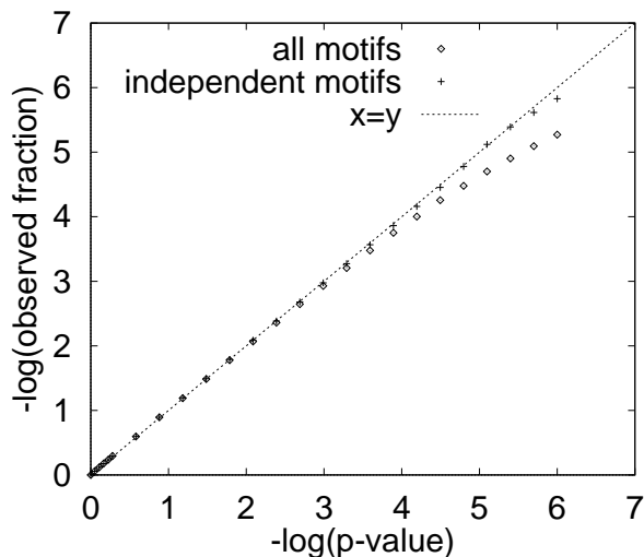
Figure 4: Accuracy of MAST p-values. The distribution of p-values estimated by MAST using the QFAST algorithm is compared with the observed distribution. The graph shows the negative logarithm of the observed fraction of sequences with the given p-value or less versus the negative logarithm of p-value. The points labeled “all motifs” are each the average of 75 experiments where five motifs characteristic of a single protein family were used to search a pseudo-random sequence database of 100,000 protein sequences of varying lengths. The points labeled “independent motifs” show the average result when all motifs that are highly similar to other motifs in their queries are removed. Points below the line x = y correspond to average p-values that overestimate the statistical significance of matches.
