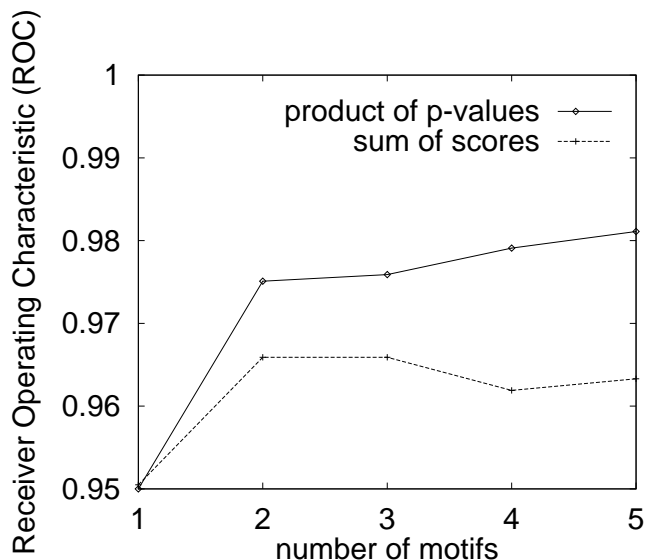
Figure 5: Classification accuracy of MAST. The curve labeled “product of p-values” shows the average classification accuracy (ROC 50 ) of the MAST algorithm when the scores of various numbers of motifs are combined using the qFAST algorithm. The other curve shows the average accuracy if the scoring function used is the sum of the match scores of the sequence and each motif in the query. Each point represents the average result of 75 distinct queries, one for each of 75 sequence families. For each family, the queries were nested: the motifs in the four-motif query were a subset of the motifs in the five-motif query, etc.
