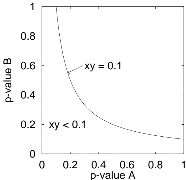
Figure 2: Using the product of p-values as a test statistic. An observed product of two p-values of 0.1 could be the result of any event whose two p-values, x and y , lie on the curve xy = 0.1 . Likewise, the probability of observing a product of two p-values less than 0.1 is the probability of all the points below the curve. If the p-values are independent and uniformly distributed, the area within the unit square beneath the curve is equal to the probability that the product is less than or equal to 0.1.
