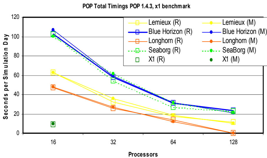
Fig. 1. Results for Parallel Ocean Program (POP). (R) is real runtime (M) is modeled (predicted) runtime
