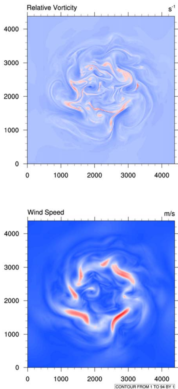
Figure 2: Relative vorticity at approximately 5 km above ground (top), and wind speed near the jet stream at approximately 10 km above ground. The entire midlatitude wave train is simulated at high resolution ( \Delta X=5 km), and the solutions show the range of scales in the flow.
