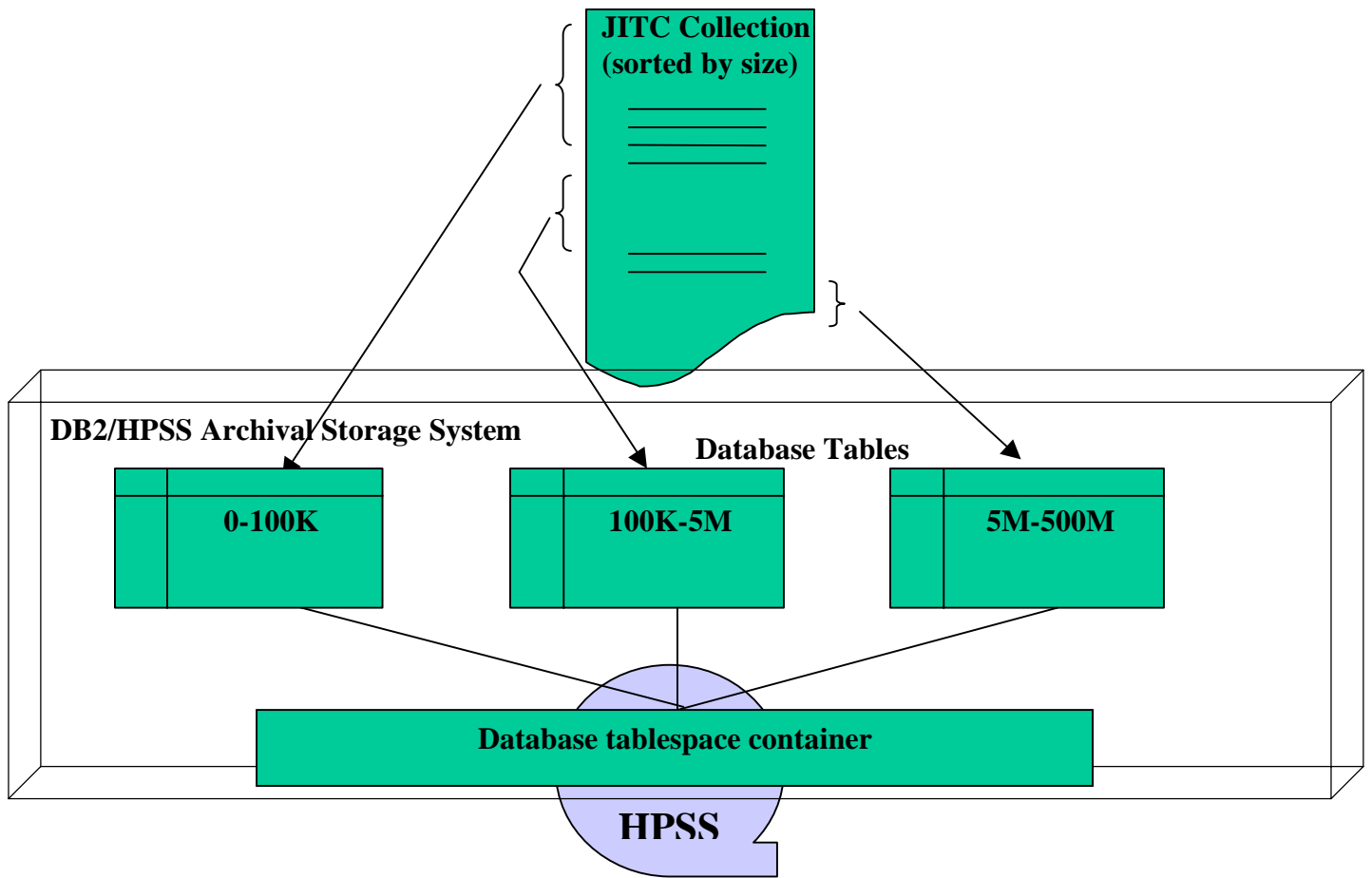
Figure 13-1. Storage strategy for the JITC collection
