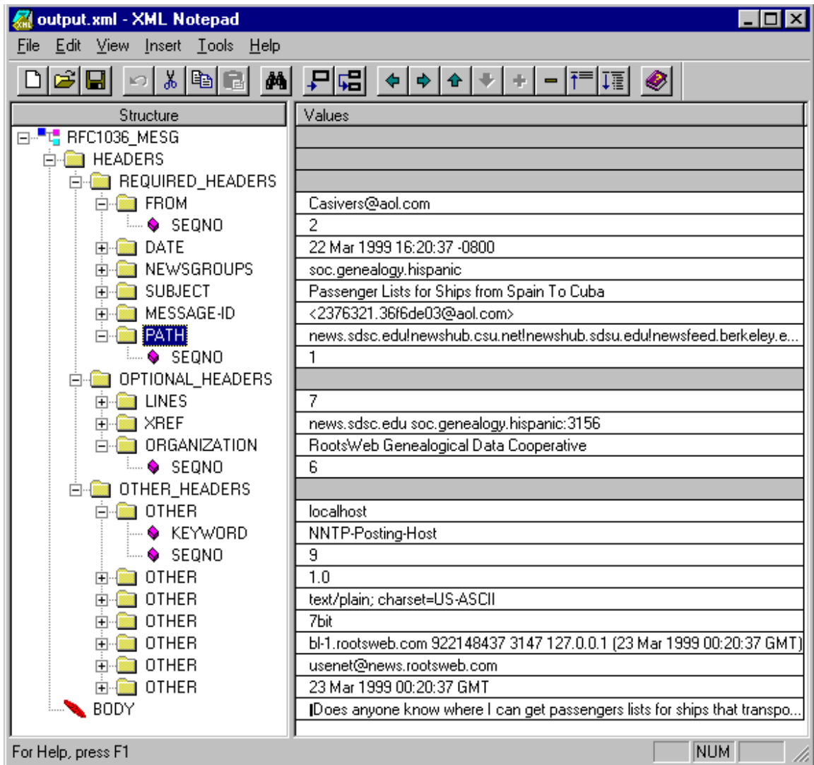
Figure 5-3. Formatted message using XML DTD
