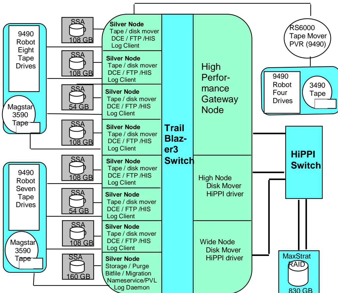
Figure 3-1. HPSS archival storage system
