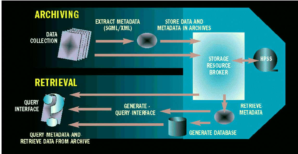
Figure 4-1. Persistent Collection Process
